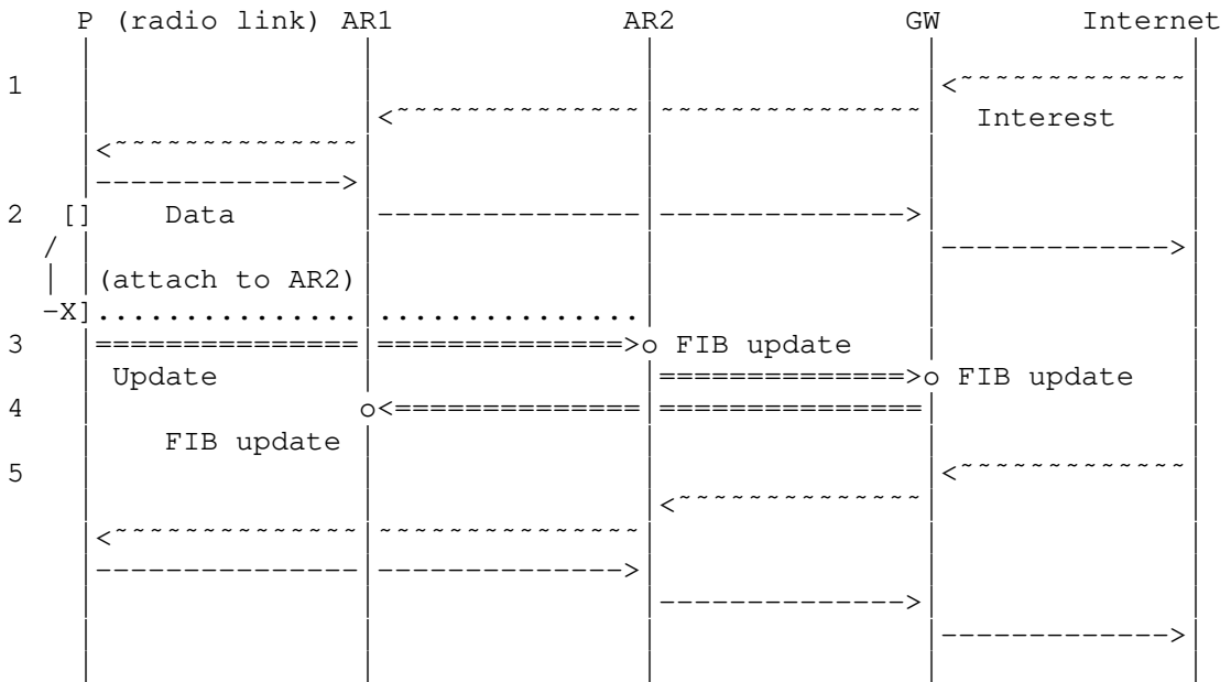
Figure 1: Signaling during producer mobility (MAP-Me)
