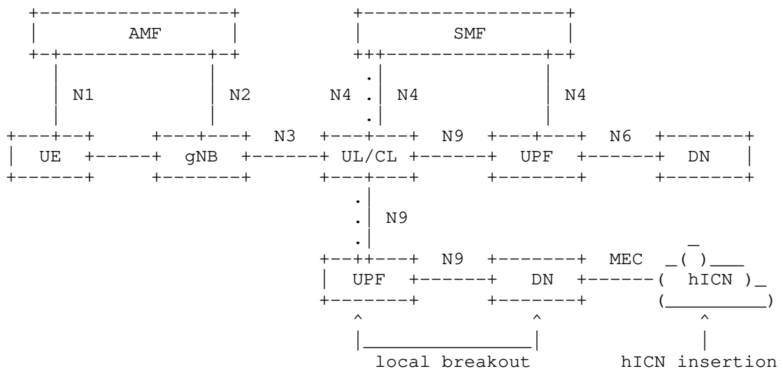
Figure 4: hICN insertion in MEC
